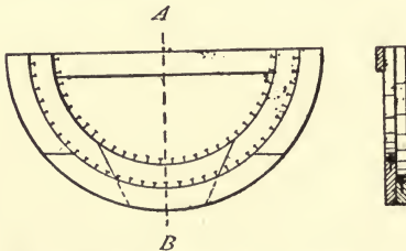
FIG. 22.—TEMPLER FOR BRICK SEWERS.
